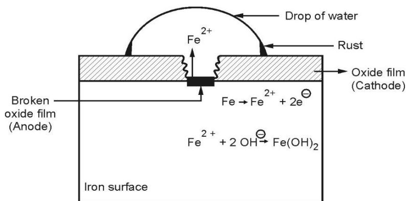
Fig. 5.2.2 Oxygen absorption mechanism
